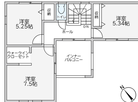
2F:51.34㎡
